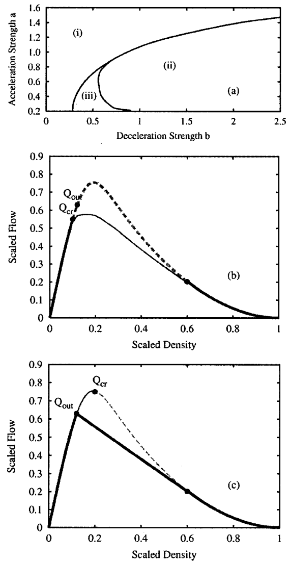
FIG. 36. Comparison of traffic models by their dynamical properties: (a) Schematic phase diagram of model classes as a function of the acceleration strength a and the deceleration strength b . (b) Models belonging to phase (i) have no critical density \rho_{cr} and display stable traffic in accordance with the fundamental diagram (heavy solid and dashed lines), while models belonging to phase (ii) show a nonhysteretic jamming transition with a resulting flow-density relation represented by solid lines. (c) A hysteretic phase transition with metastable high-flow states is found for models belonging to phase (iii). The model behavior is determined by the relative magnitude of the outflow Q_{out} from congested traffic compared to the flow Q_{cr} = Q_e(\rho_{cr}) at which traffic becomes linearly unstable with respect to small perturbations. After Krauß, 1998a.
