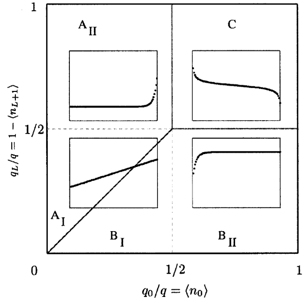
FIG. 32. Phase diagram of the totally asymmetric simple exclusion process (TASEP) with open boundaries and of other models that can be macroscopically described by the Lighthill-Whitham or Burgers equation, with representative density profiles (see insets). The diagonal line separates the areas A_I and A_{II} of downstream shock propagation from the areas B_I and B_{II} of upstream shock propagation with corresponding changes in the density profile. Consequently crossing this line is related to a transition between a low-density phase controlled by the upstream boundary and a high-density phase controlled by the downstream boundary. Area C is characterized by the maximum possible flow. After Schütz and Domany, 1993; Schütz, 2000a.
