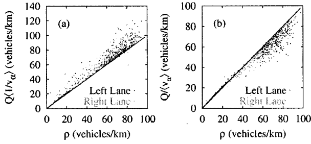
FIG. 26. Fifty-vehicle averages of (a) the density Q\langle 1/v_\alpha \rangle and (b) the conventionally determined density Q\langle v_\alpha \rangle , both as a function of the density \rho according to the proposed definition (14). The usually assumed relations are indicated by solid lines. From Tilch and Helbing, 2000.
