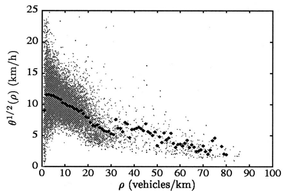
FIG. 14. Density-dependent standard deviation \sqrt{\theta} of vehicle velocities in a single lane of the freeway: Fine dots, 1-minute data; ♦, average values for a given density \rho . The velocity variance \theta is more or less monotonically falling with increasing density. The greater scattering above 30 vehicles per kilometer indicates unstable traffic flows. After Helbing, 1997a, 1997b, 1997e.
